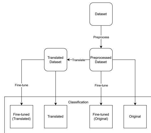
Figure 1: Evaluation methodology of machine translation-based hate speech detection.
